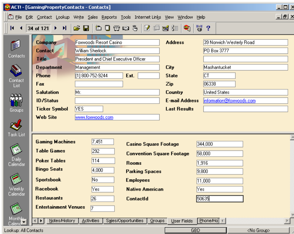
Figure 3: ACT!2000 Contact Record Displayed Using the GBD Layout
